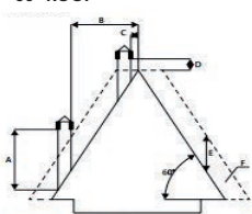
60° ROOF
