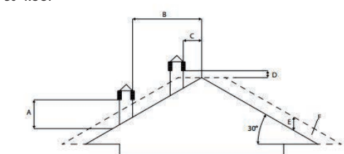
30° ROOF
