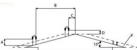
TECHO A 15°
