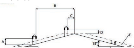
15° ΟΡΟΦΗ
